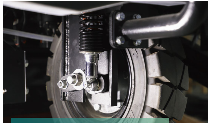
Wheels are equipped with shock absorption system, which can easily pass through the uneven road. Driving is more comfortable
